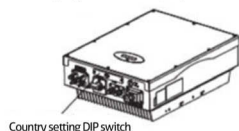
Country setting DIP switch
